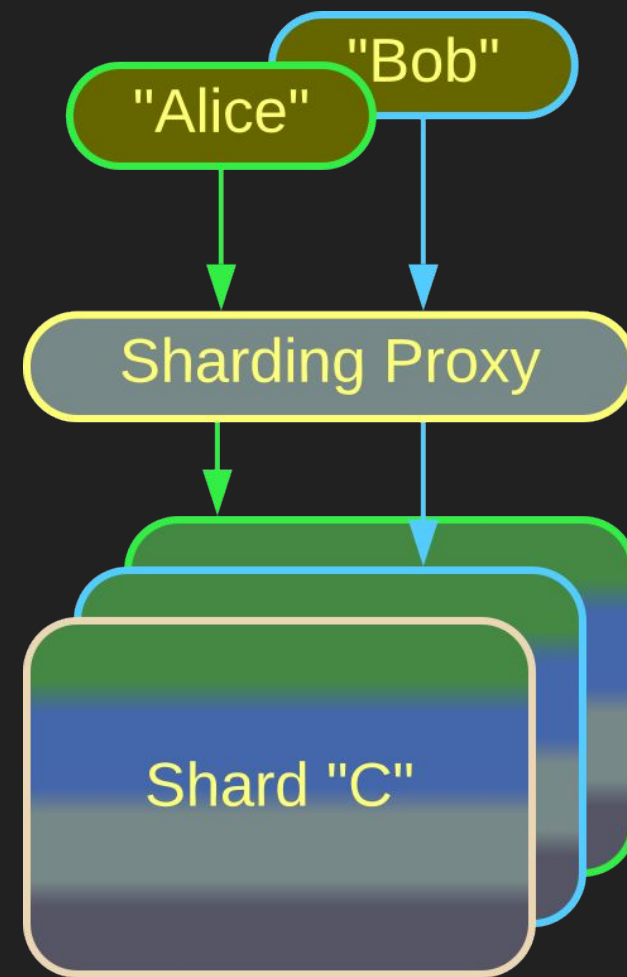
Shards, Partitions
