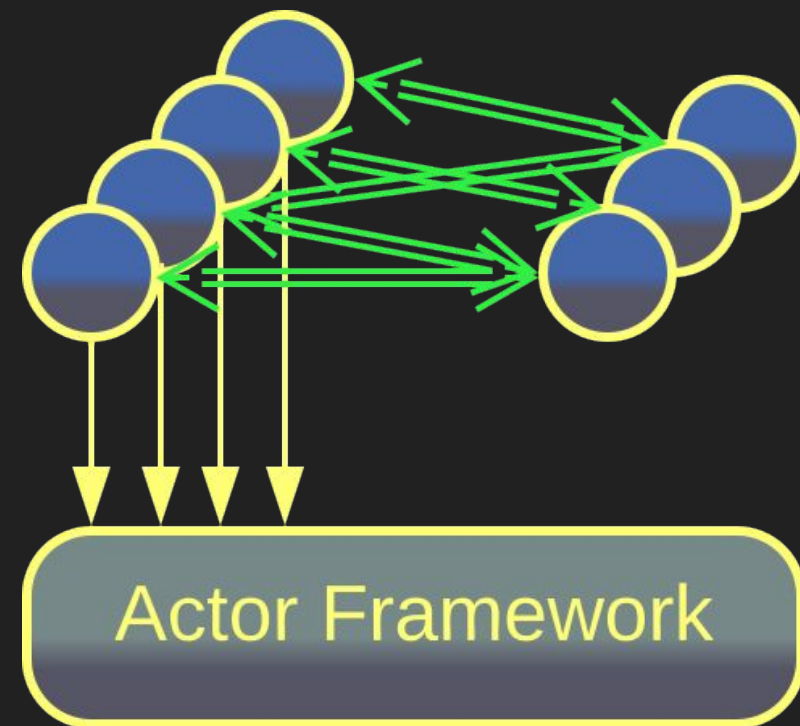
Actors
