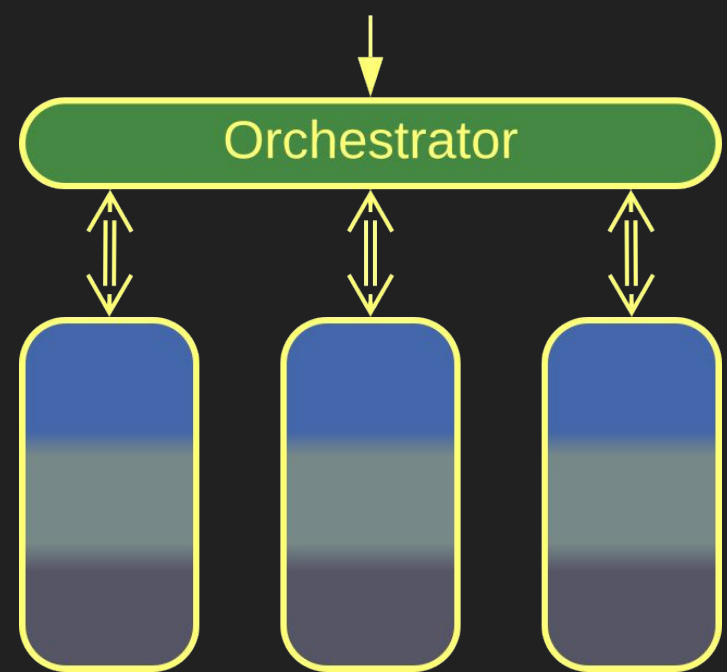
Orchestrated Services
