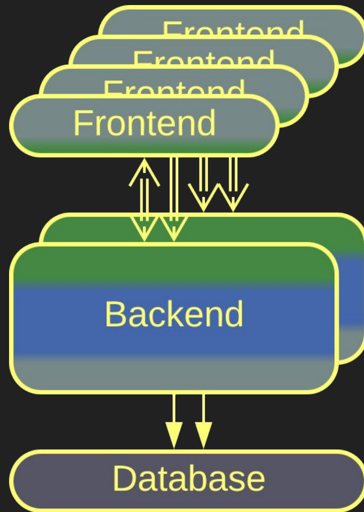
3-Tier system
