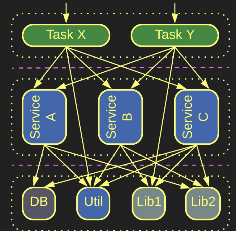
Service-Oriented Architecture
