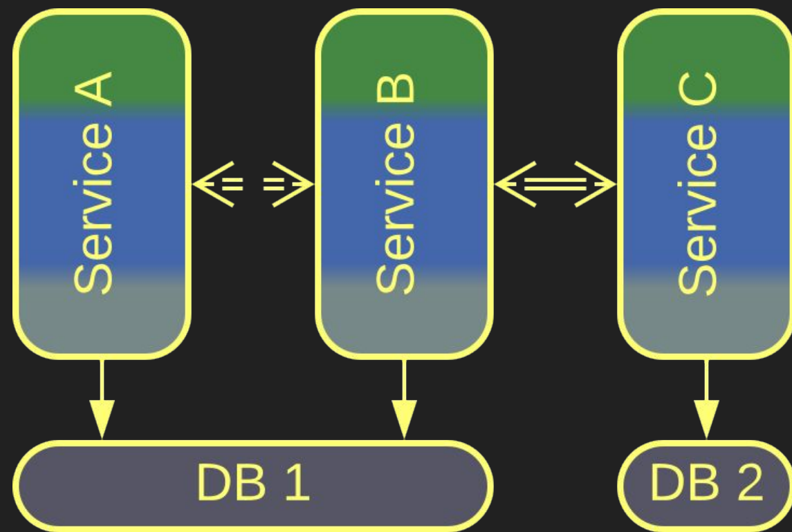
Service-Based Architecture
